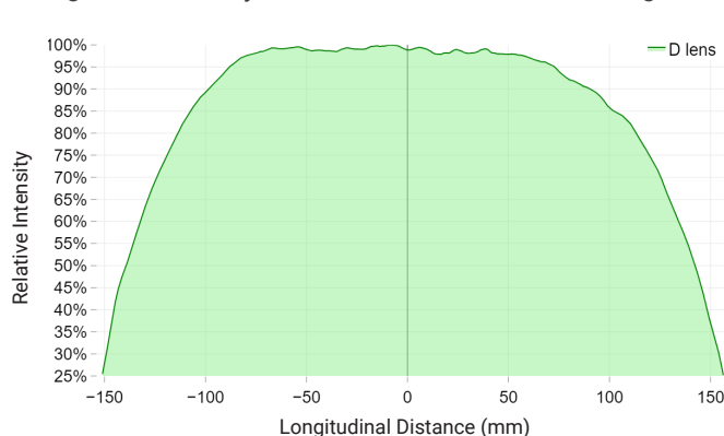
Longitudinal Intensity Distribution Profile at 50 mm Working Distance
