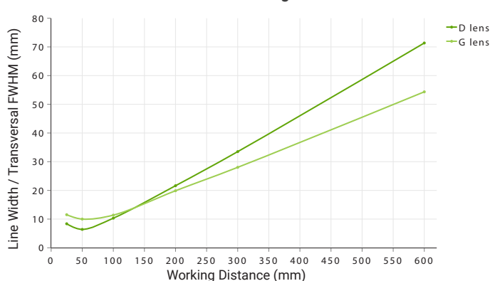
Line Width vs Working Distance
