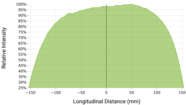
Line Intensity Distribution Profile at 25 mm Working Distance
