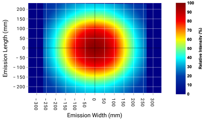
Intensity distribution sample image was taken with a 12-inch white DL067 unit.
