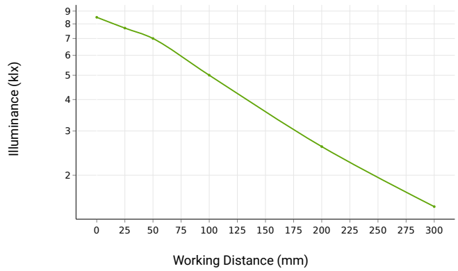
Illuminance data was collected using a 12-inch white DL067 unit.
