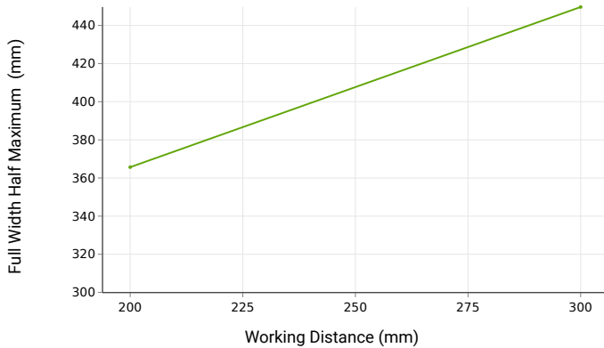
Full Width Half Maximum (FWHM) data collected using a white DL067 unit.
