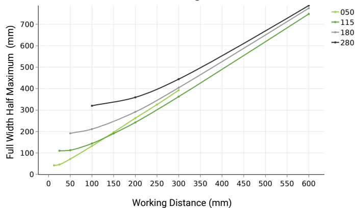
FWHM vs Working Distance
