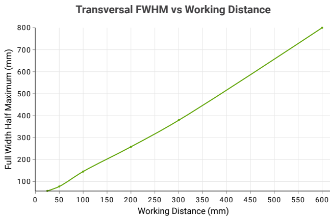
Both Full Width Half Maximum (FWHM) vs Working Distance plots shown above have been measured using a 12-inch white AL116 unit.
