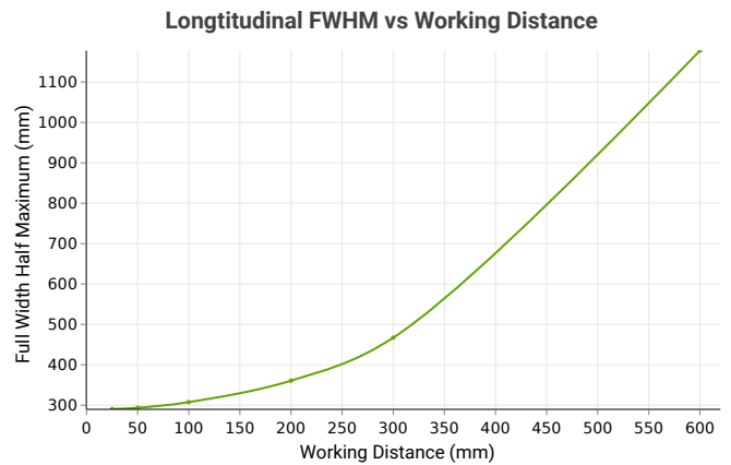
Both Full Width Half Maximum (FWHM) vs Working Distance plots shown above have been measured using a 12-inch white AL116 unit.
