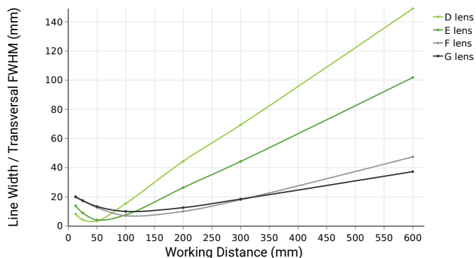
Line Width vs Working Distance
