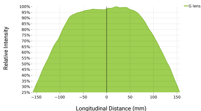
Longitudinal Intensity Distribution Profile at 50 mm Working Distance
