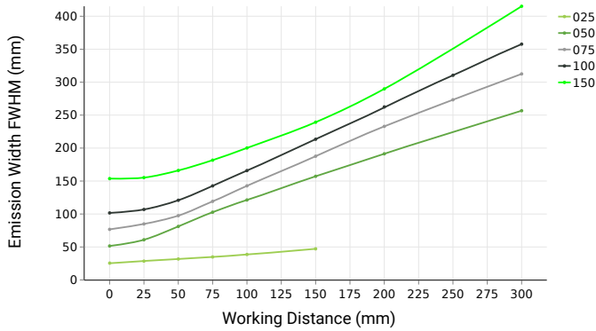
FWHM data was collected using white DL225 units.
