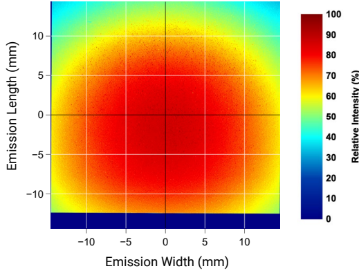
Intensity distribution sample image was taken with a 25 mm white DL225 unit.
