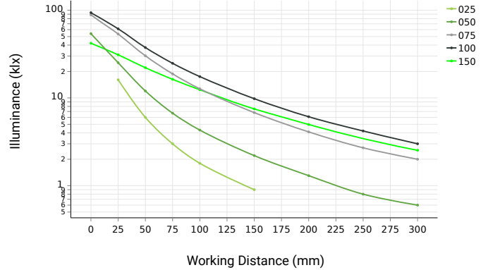
Illuminance data was collected using white DL225 units.
