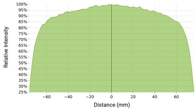
Emission Width Profile Plot sample was taken with a 25 mm white DL225 unit at a 25mm working distance.
