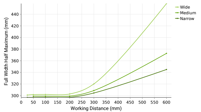
Both Full Width Half Maximum (FWHM) vs Working Distance plots shown above have been measured using a 12-inch white AL247 unit.
