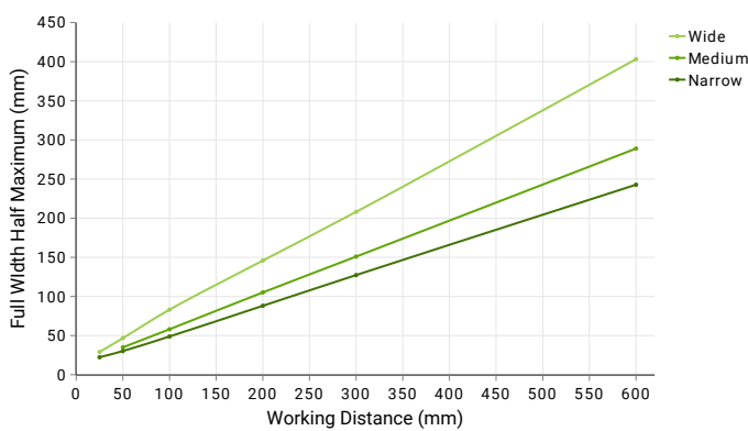
Both Full Width Half Maximum (FWHM) vs Working Distance plots shown above have been measured using a 12-inch white AL247 unit.
