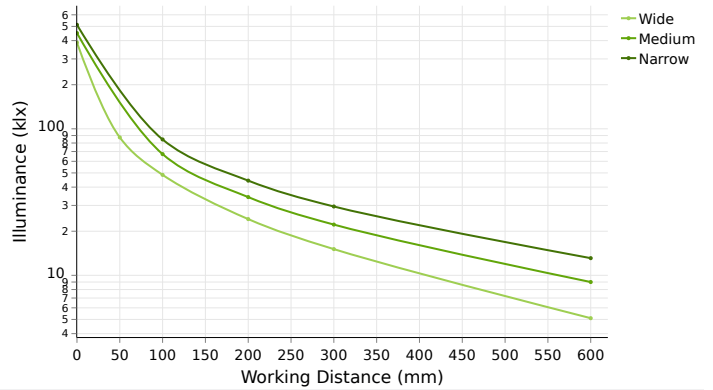
Data shown above have been collected using a 12-inch white AL247 unit.
