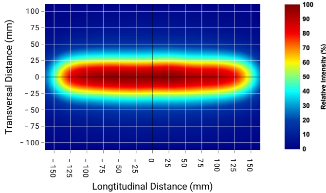
Intensity distribution sample image above taken with a 12-inch white medium lensed AL247 unit.
